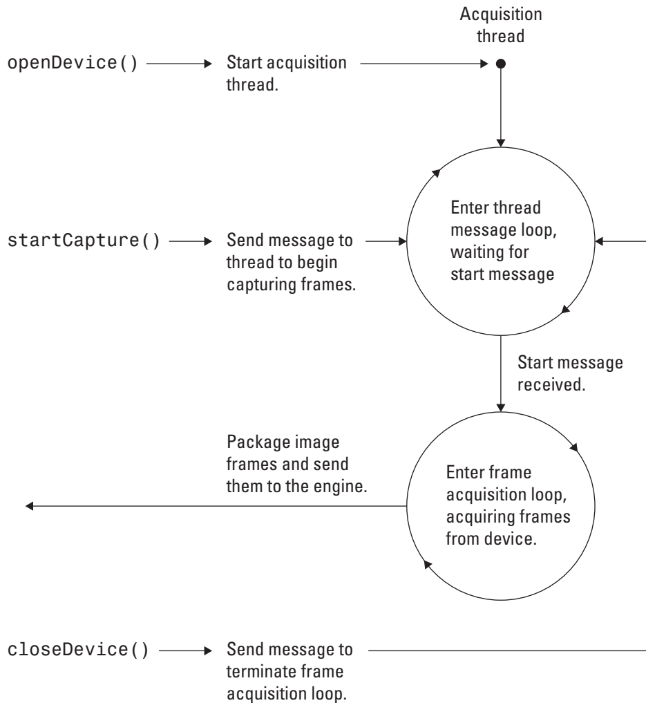
Interaction of Adaptor Functions and Acquisition Thread
